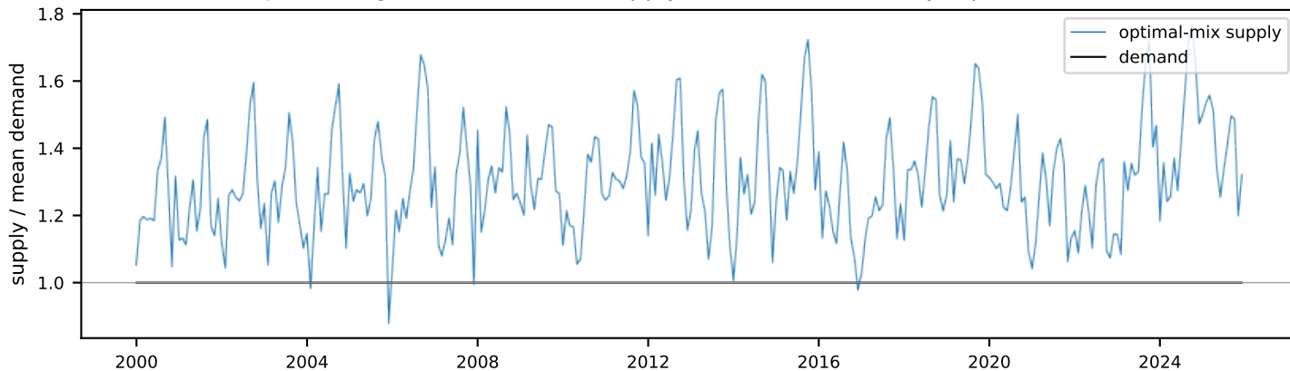
Jawa Tengah — normalized supply vs demand (monthly, optimal mix)
