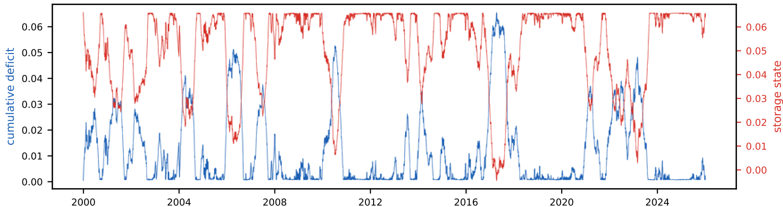
Cumulative deficit & storage state (peak deficit = required storage, S_{\text{tot}} =6.6% of annual)
