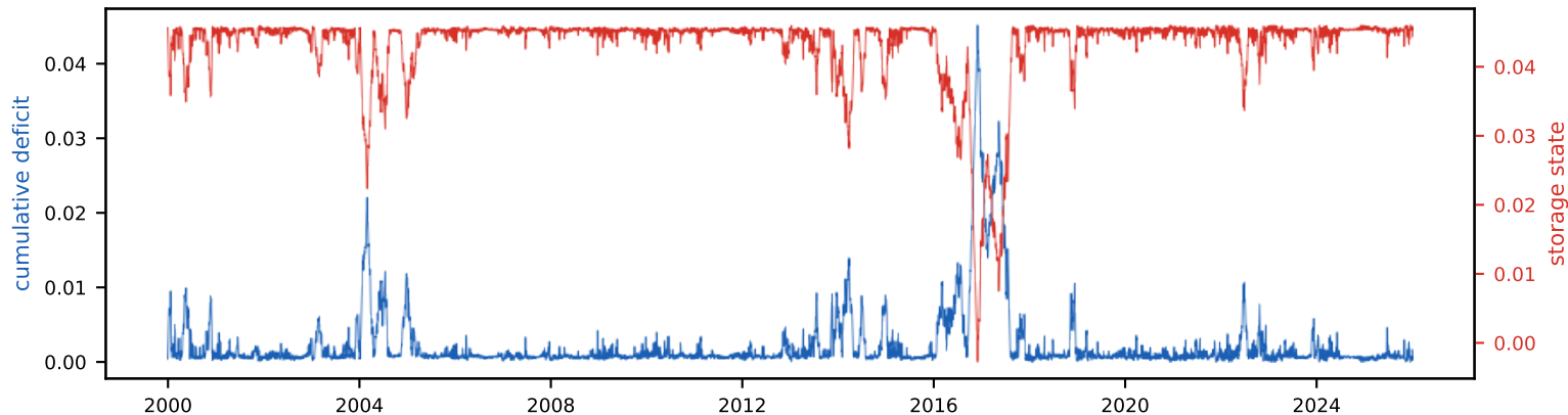
Cumulative deficit & storage state (peak deficit = required storage, S_{tot}=4.6\% of annual)
