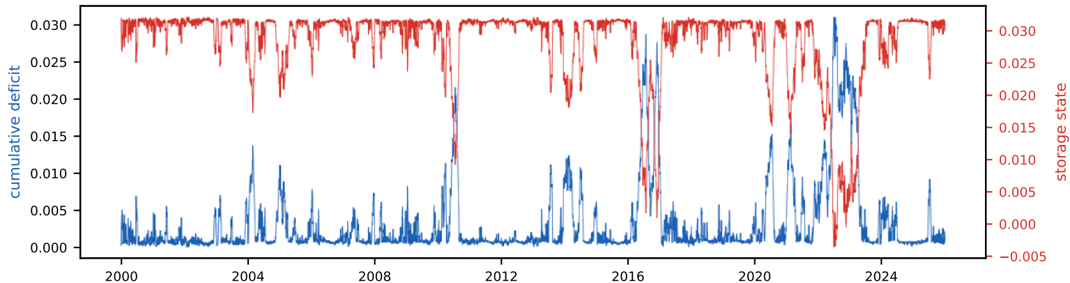
Cumulative deficit & storage state (peak deficit = required storage, S_{\text{tot}} =3.2% of annual)
