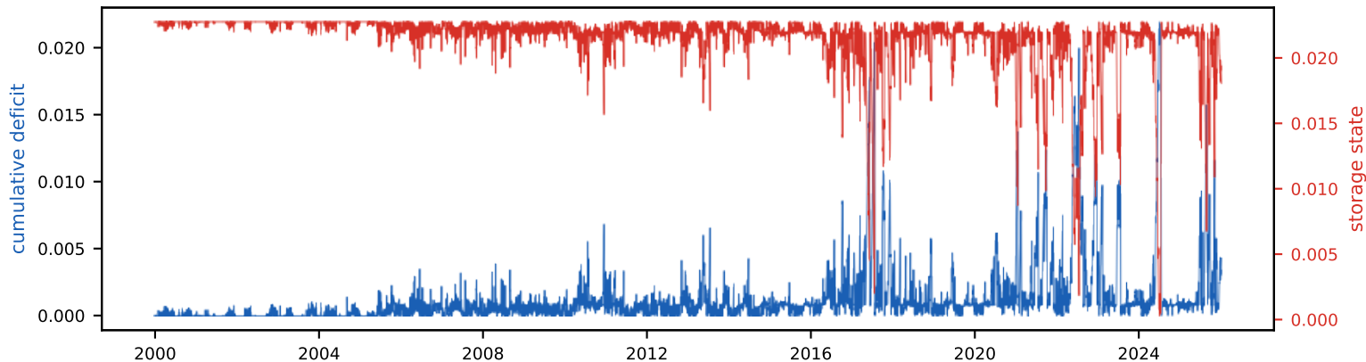
Cumulative deficit & storage state (peak deficit = required storage, S_{\text{tot}} =2.3% of annual)
