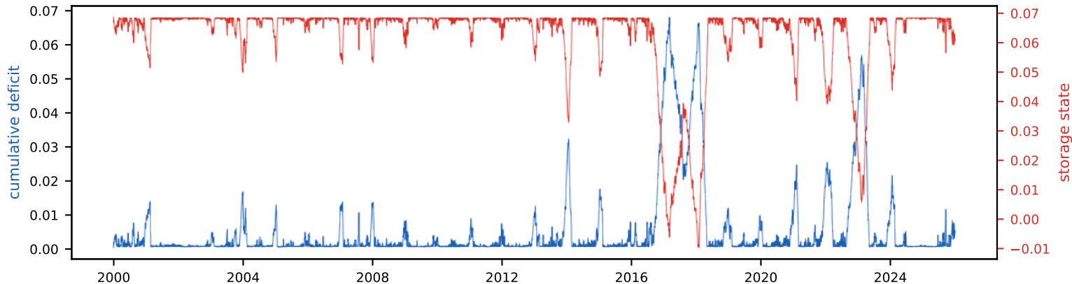
Cumulative deficit & storage state (peak deficit = required storage, S_{\text{tot}} =6.9% of annual)
