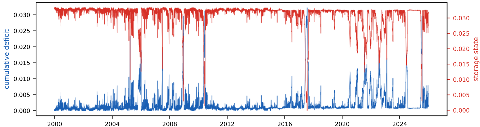
Cumulative deficit & storage state (peak deficit = required storage, S_{\text{tot}} =3.3% of annual)
