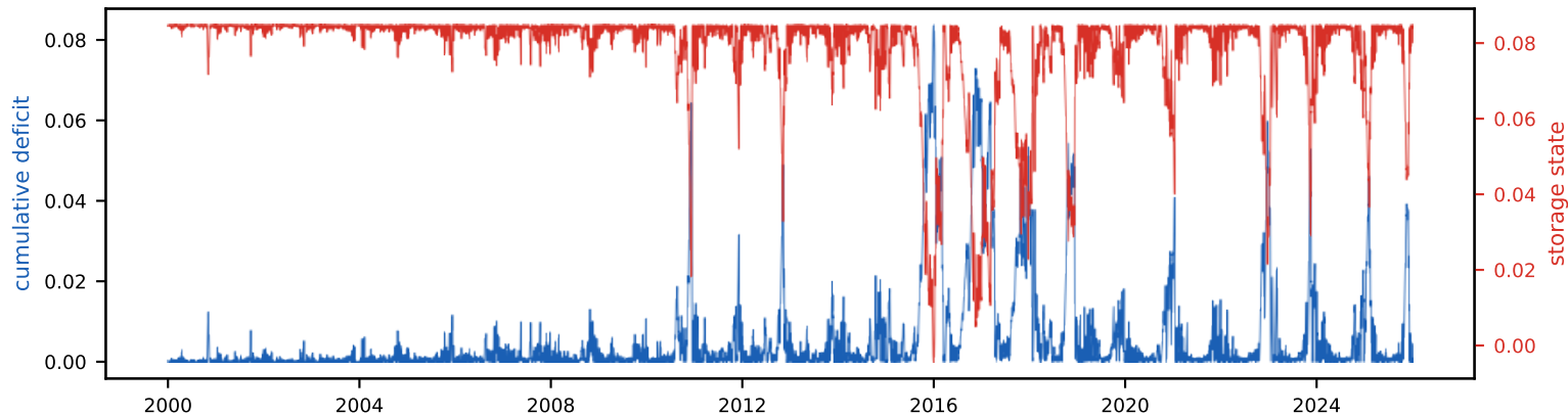
Cumulative deficit & storage state (peak deficit = required storage, S_{\text{tot}} =8.5% of annual)
