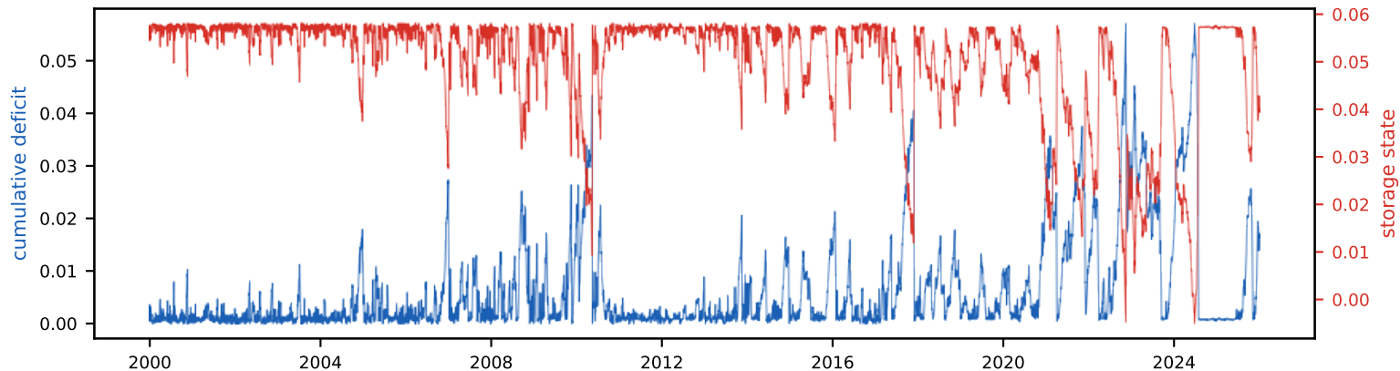
Cumulative deficit & storage state (peak deficit = required storage, S_{tot} =5.8% of annual)
