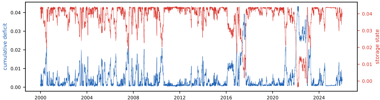
Cumulative deficit & storage state (peak deficit = required storage, S_{\text{tot}} =4.5% of annual)
