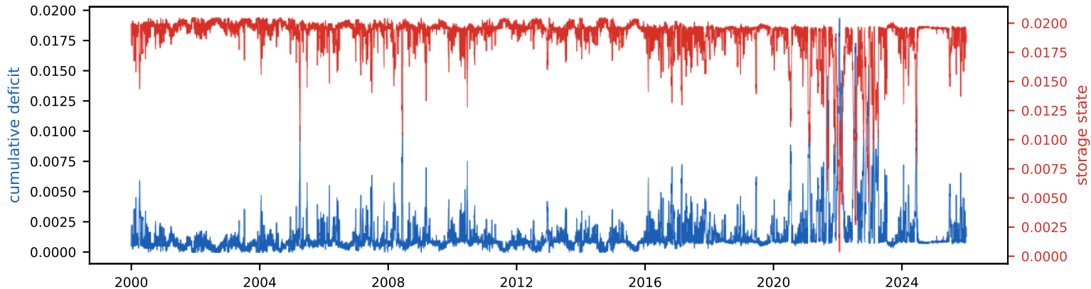
Cumulative deficit & storage state (peak deficit = required storage, S_{\text{tot}} =2.0% of annual)
