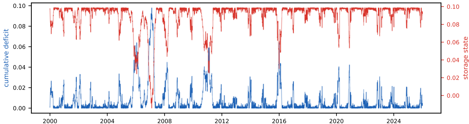
Cumulative deficit & storage state (peak deficit = required storage, S_{\text{tot}} =9.9% of annual)
