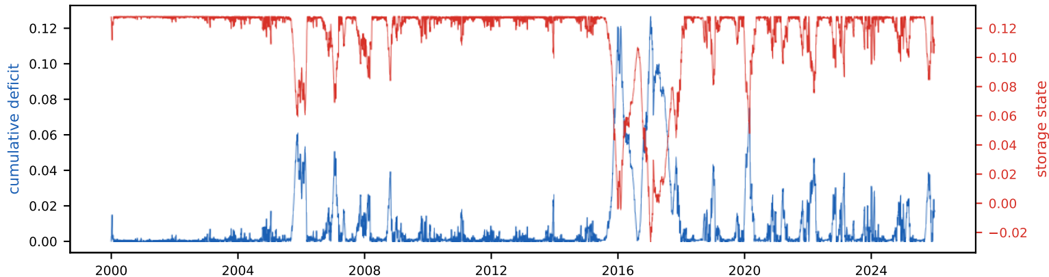
Cumulative deficit & storage state (peak deficit = required storage, S_{\text{tot}} =12.8% of annual)
