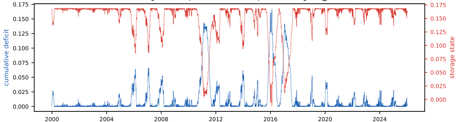
Cumulative deficit & storage state (peak deficit = required storage, S_{\text{tot}} =16.8% of annual)
