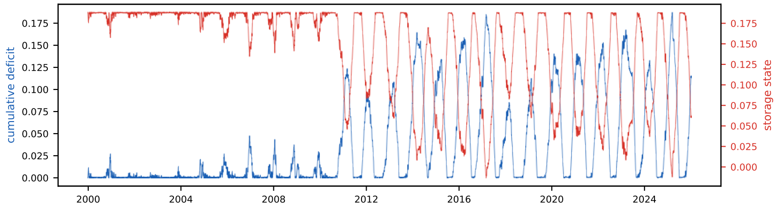
Cumulative deficit & storage state (peak deficit = required storage, S_{\text{tot}} =18.8% of annual)
