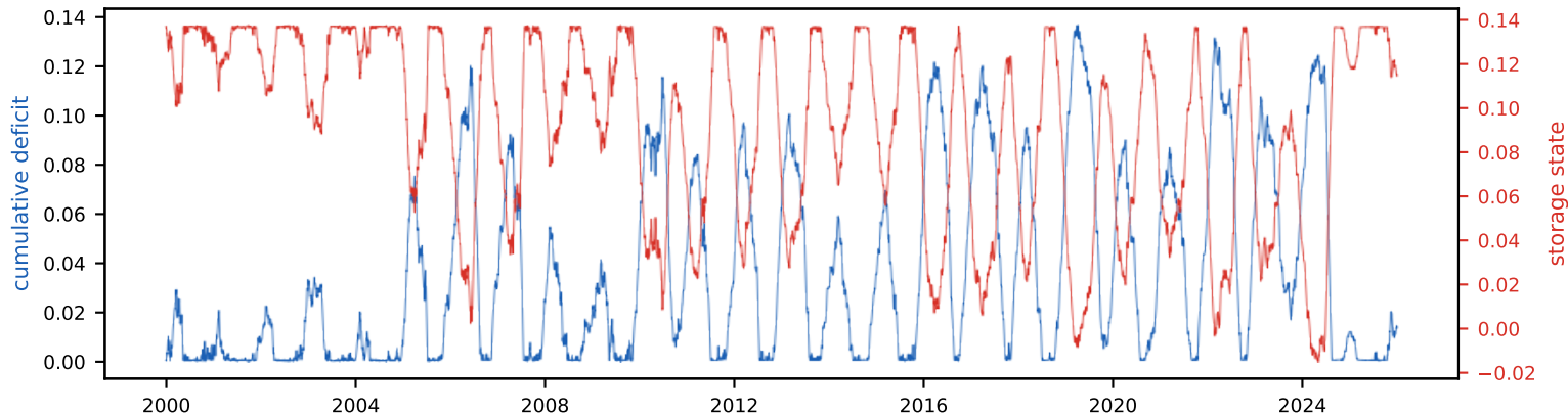
Cumulative deficit & storage state (peak deficit = required storage, S_{\text{tot}} =13.7% of annual)
