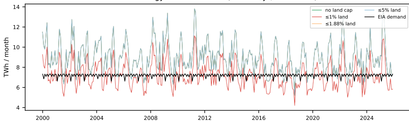
Real energy vs EIA demand (86 TWh/yr, 1.2% land)
