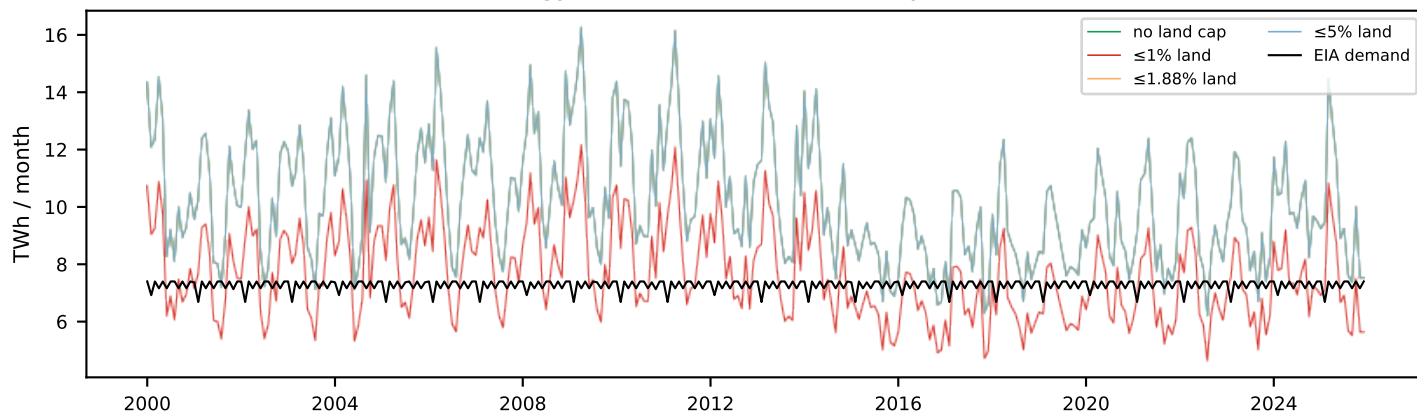
Real energy vs EIA demand (87 TWh/yr, 1.3% land)
