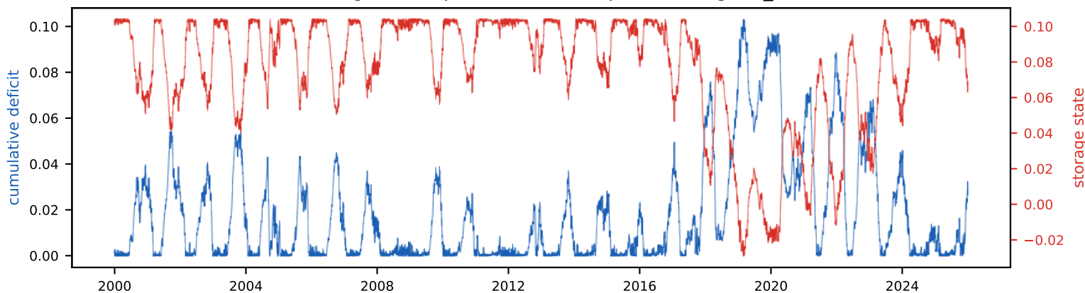
Real energy vs EIA demand (135 TWh/yr, 1.7% land)
