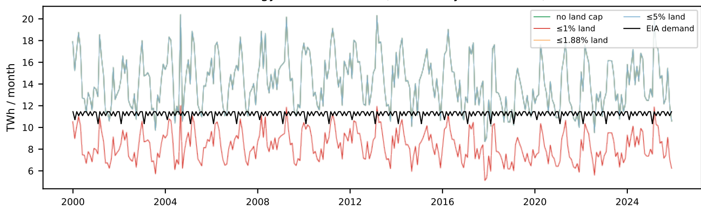
Real energy vs EIA demand (135 TWh/yr, 1.7% land)
