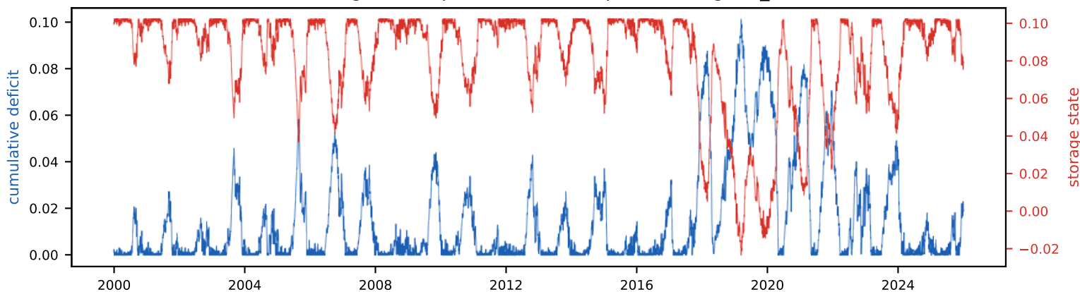
Real energy vs EIA demand (80 TWh/yr, 1.7% land)
