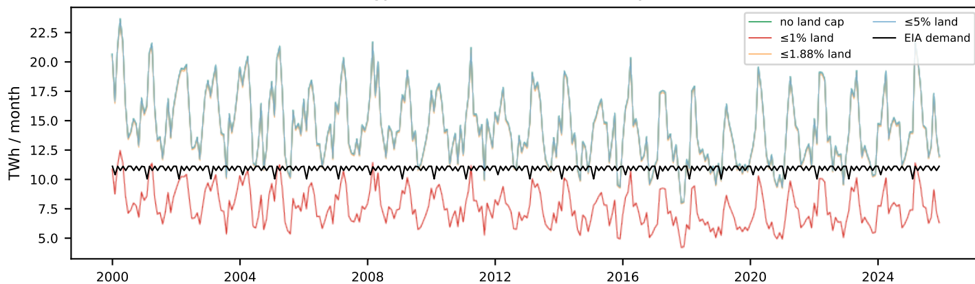
Real energy vs EIA demand (131 TWh/yr, 1.9% land)
