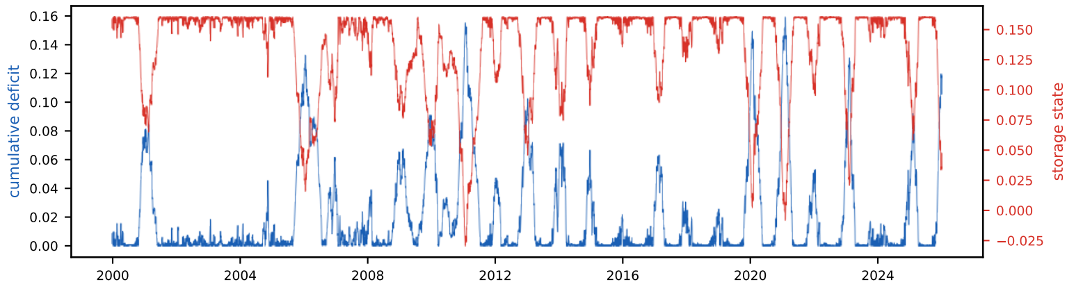
Cumulative deficit & storage state (peak deficit = required storage, S_{\text{tot}} =16.0% of annual)
