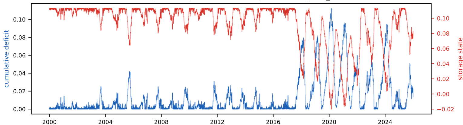
Real energy vs EIA demand (11 TWh/yr, 110.9% land)
