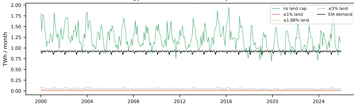
Real energy vs EIA demand (11 TWh/yr, 110.9% land)
