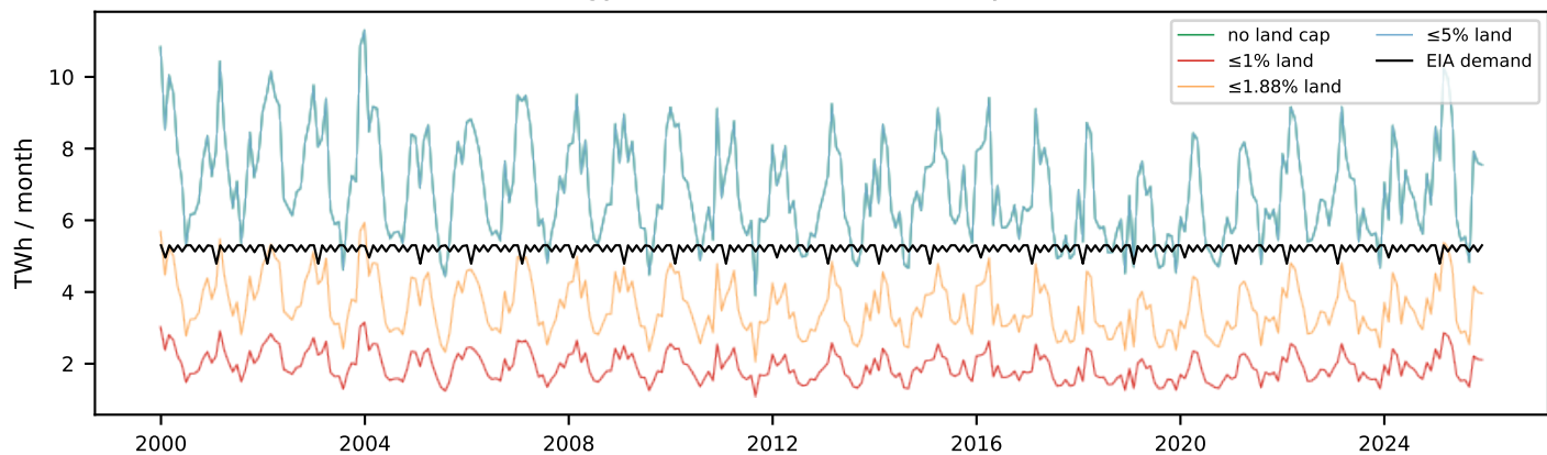
Real energy vs EIA demand (62 TWh/yr, 3.6% land)
