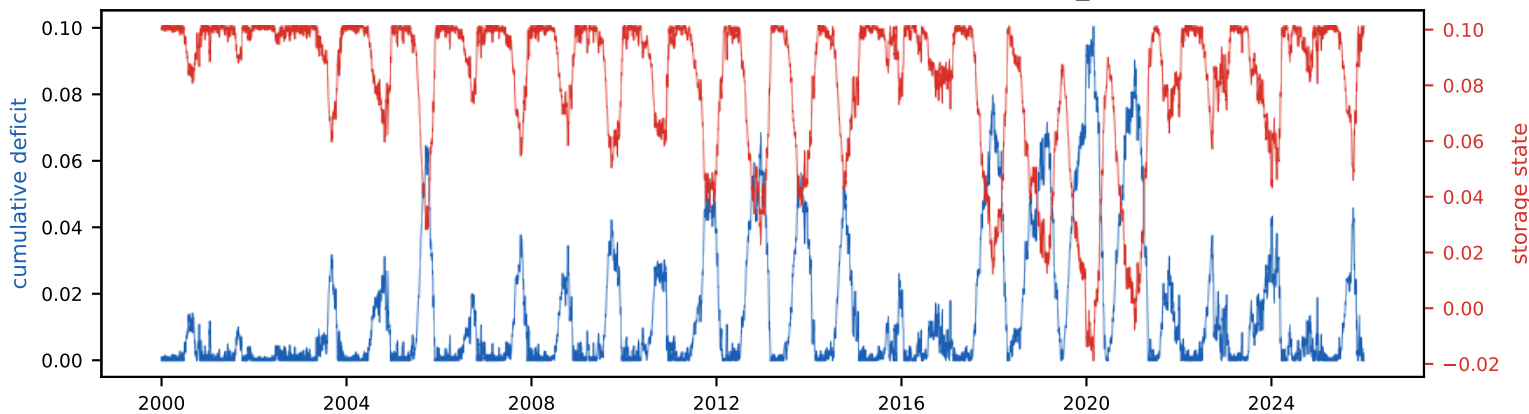
Real energy vs EIA demand (62 TWh/yr, 3.6% land)
