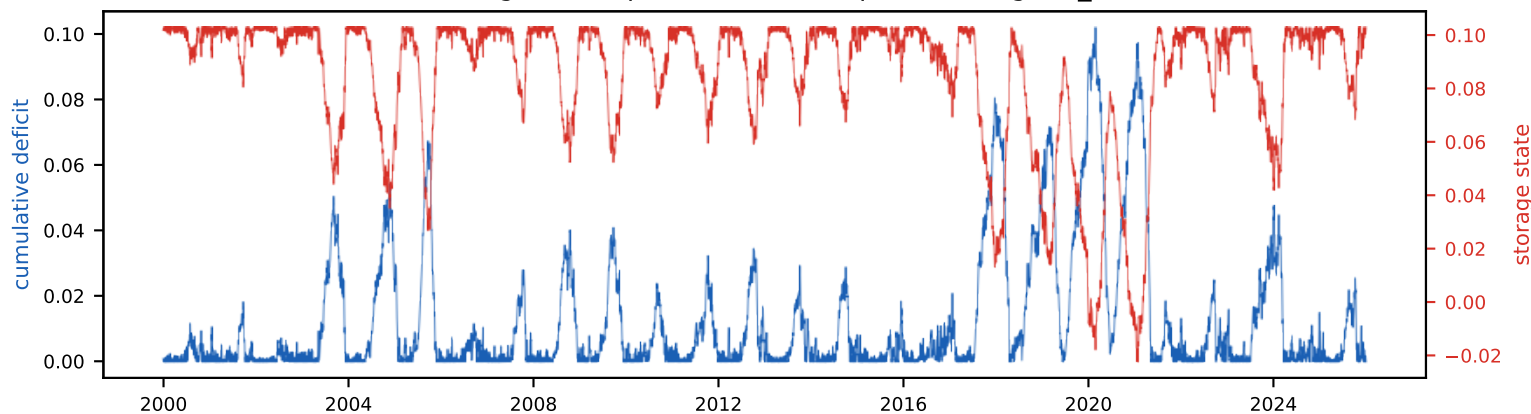
Real energy vs EIA demand (12 TWh/yr, 2.7% land)
