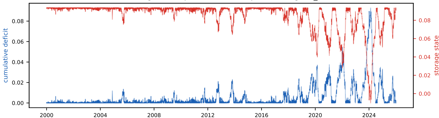
Real energy vs EIA demand (8 TWh/yr, 3.7% land)
