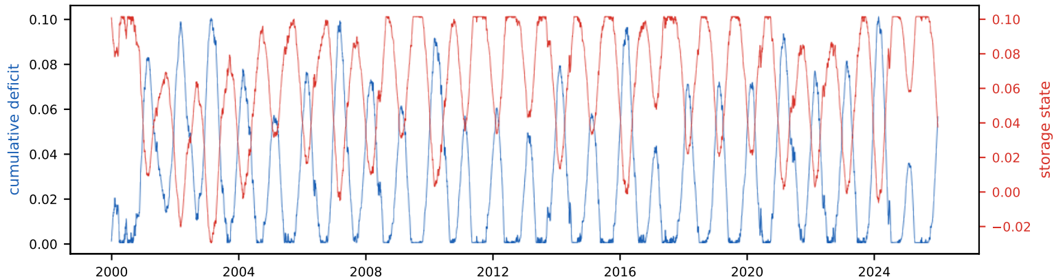
Cumulative deficit & storage state (peak deficit = required storage, S_{\text{tot}} =10.2% of annual)
