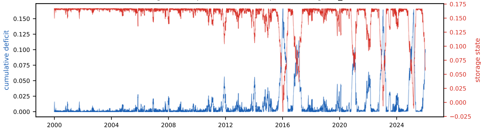
Cumulative deficit & storage state (peak deficit = required storage, S_{\text{tot}} =16.7% of annual)
