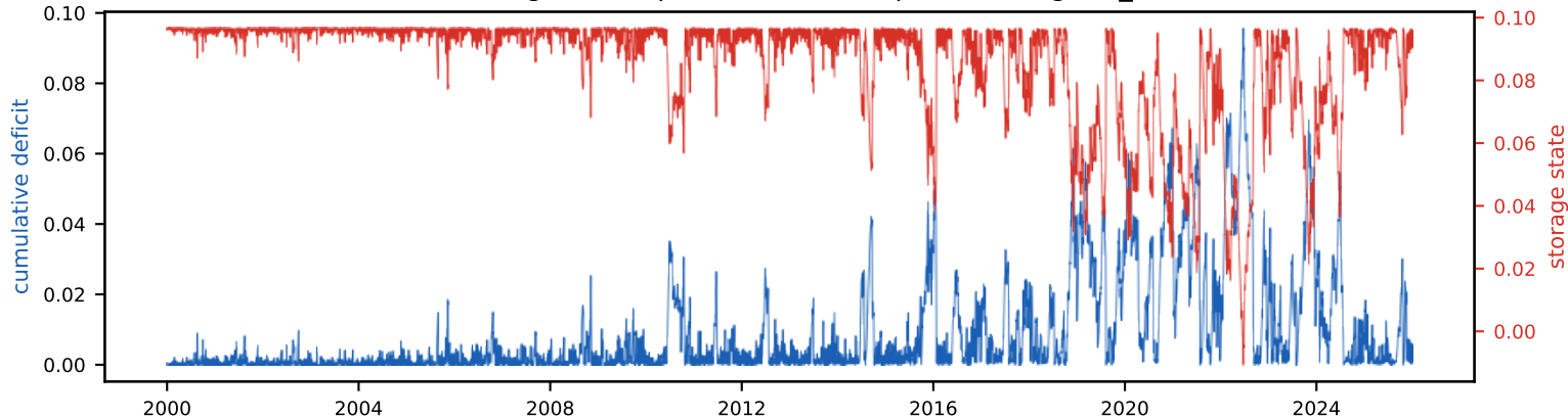
Cumulative deficit & storage state (peak deficit = required storage, S_{\text{tot}} =9.7% of annual)
