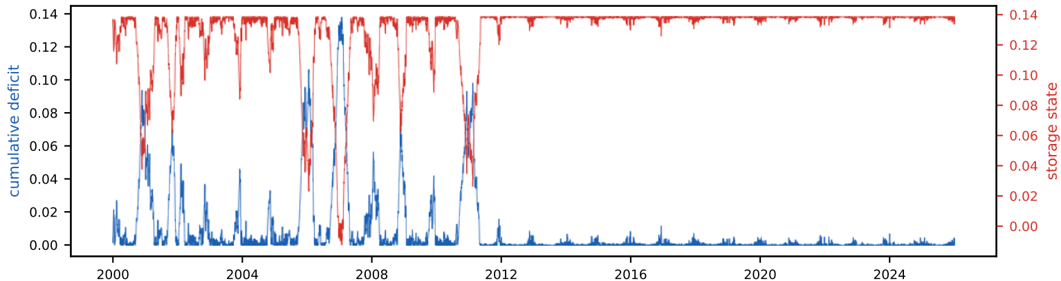
Cumulative deficit & storage state (peak deficit = required storage, S_{\text{tot}} =13.8% of annual)
