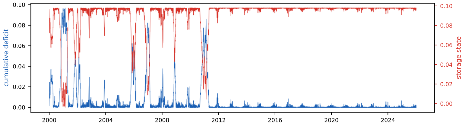
Cumulative deficit & storage state (peak deficit = required storage, S_{tot} =9.8% of annual)
