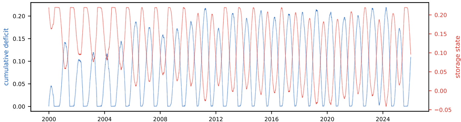
Cumulative deficit & storage state (peak deficit = required storage, S_{\text{tot}} =22.0% of annual)
