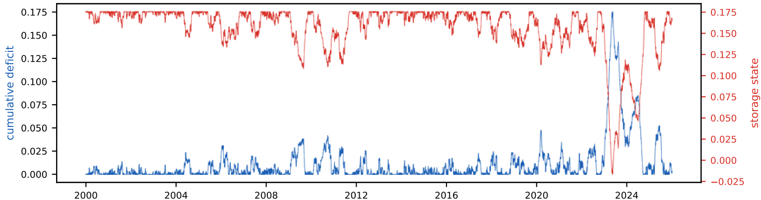
Cumulative deficit & storage state (peak deficit = required storage, S_{\text{tot}} =17.5% of annual)
