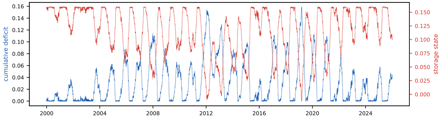
Cumulative deficit & storage state (peak deficit = required storage, S_{\text{tot}} =15.9% of annual)
