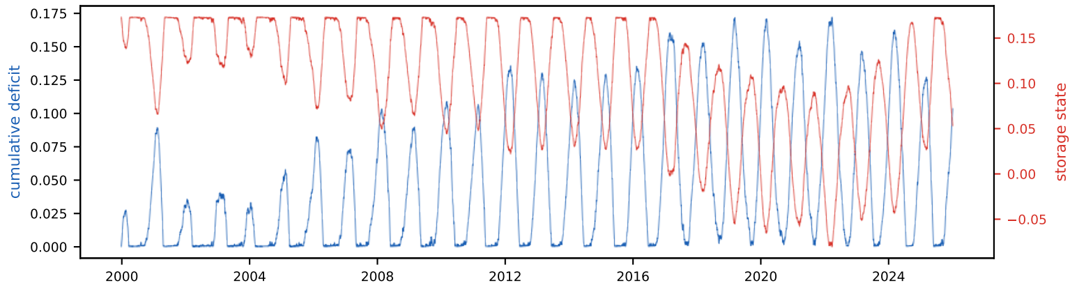
Cumulative deficit & storage state (peak deficit = required storage, S_{\text{tot}} =17.3% of annual)
