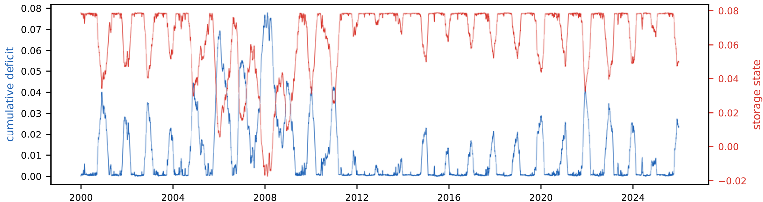
Cumulative deficit & storage state (peak deficit = required storage, S_{tot}=7.9\% of annual)
