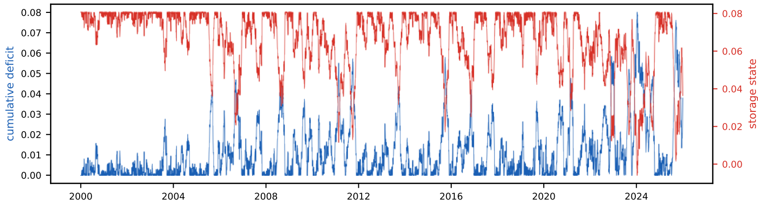
Cumulative deficit & storage state (peak deficit = required storage, S_{\text{tot}} =8.1% of annual)
