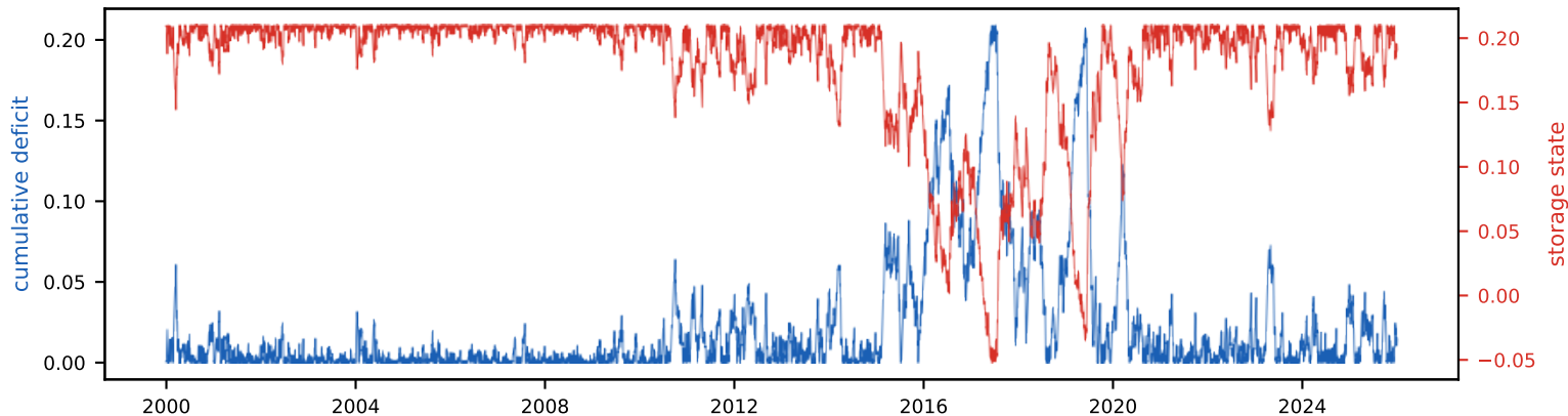
Cumulative deficit & storage state (peak deficit = required storage, S_{\text{tot}} =21.0% of annual)
