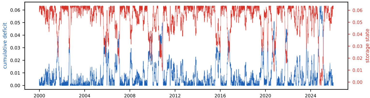
Cumulative deficit & storage state (peak deficit = required storage, S_{\text{tot}} =6.3% of annual)
