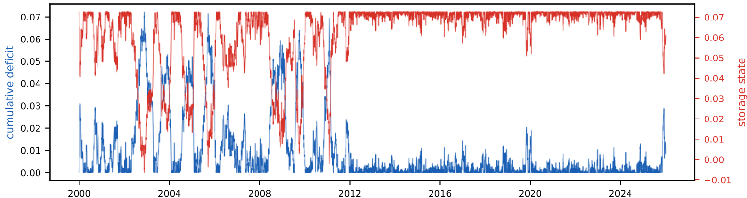
Cumulative deficit & storage state (peak deficit = required storage, S_{\text{tot}} =7.2% of annual)
