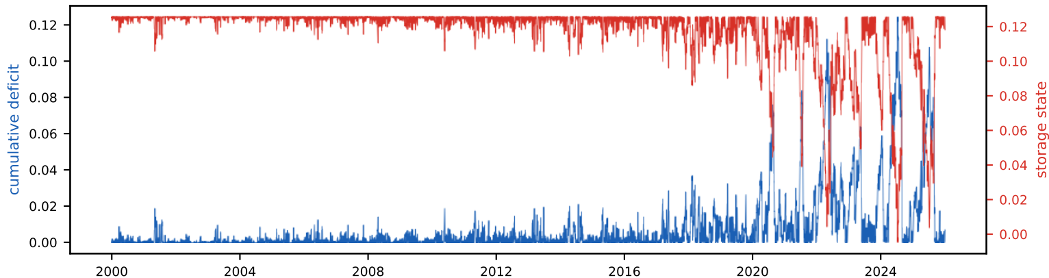
Cumulative deficit & storage state (peak deficit = required storage, S_{\text{tot}} =12.5% of annual)
