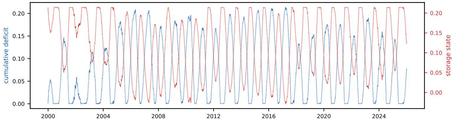
Cumulative deficit & storage state (peak deficit = required storage, S_{\text{tot}} =21.5% of annual)
