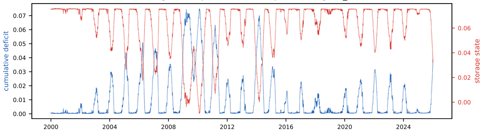
Real energy vs EIA demand (10 TWh/yr, 1.1% land)
