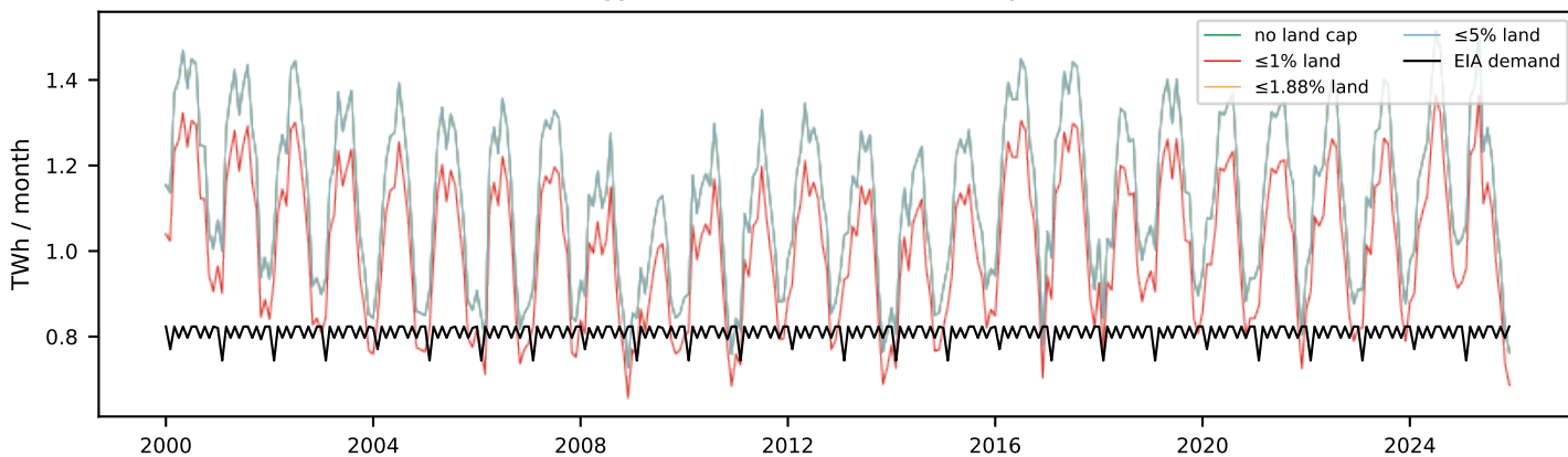
Real energy vs EIA demand (10 TWh/yr, 1.1% land)
