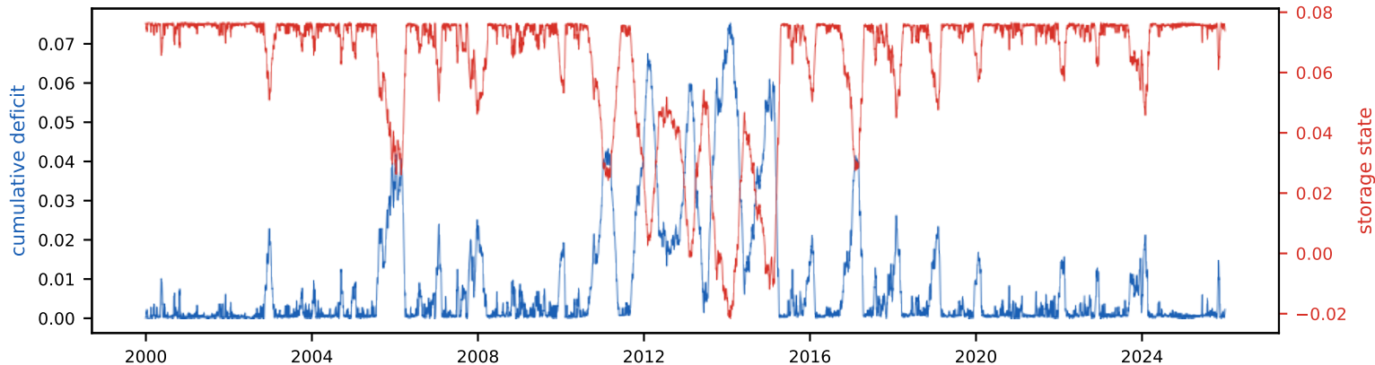
Cumulative deficit & storage state (peak deficit = required storage, S_{\text{tot}} =7.6% of annual)
