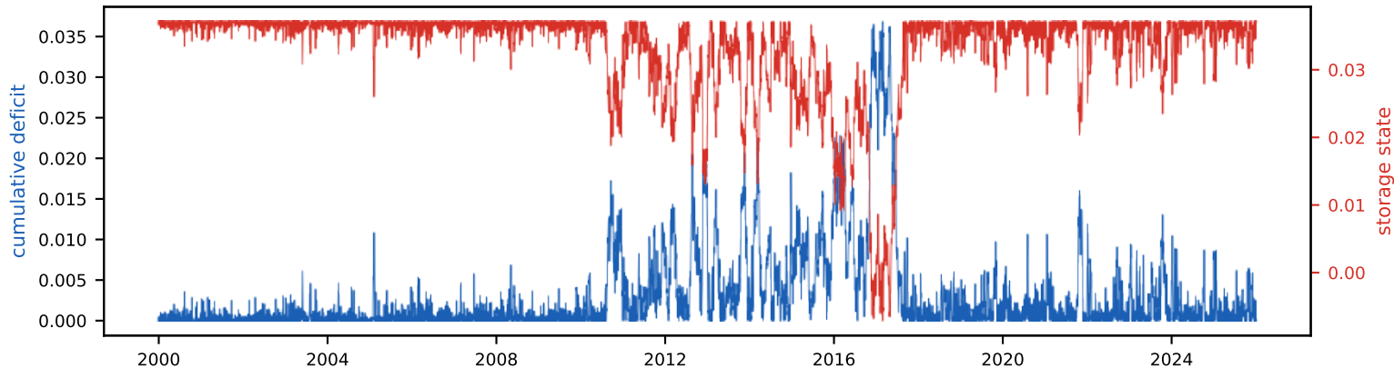
Cumulative deficit & storage state (peak deficit = required storage, S_{\text{tot}} =3.7% of annual)
