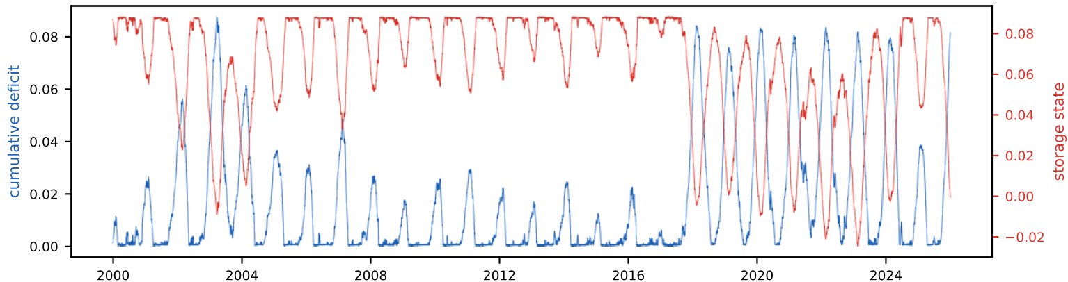
Cumulative deficit & storage state (peak deficit = required storage, S_{\text{tot}} =8.8% of annual)
