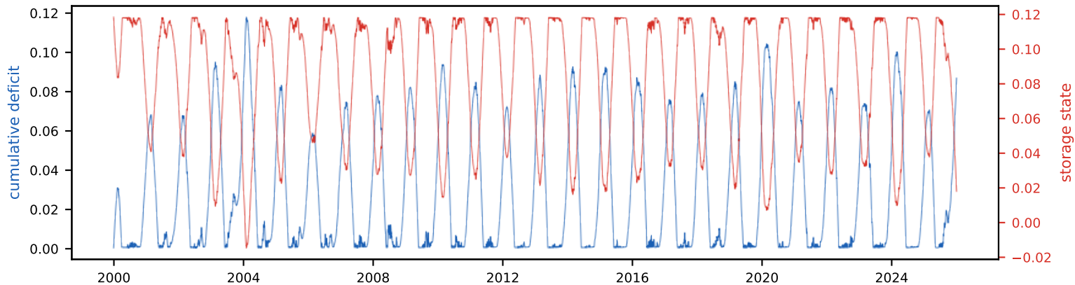
Cumulative deficit & storage state (peak deficit = required storage, S_{\text{tot}} =11.9% of annual)
