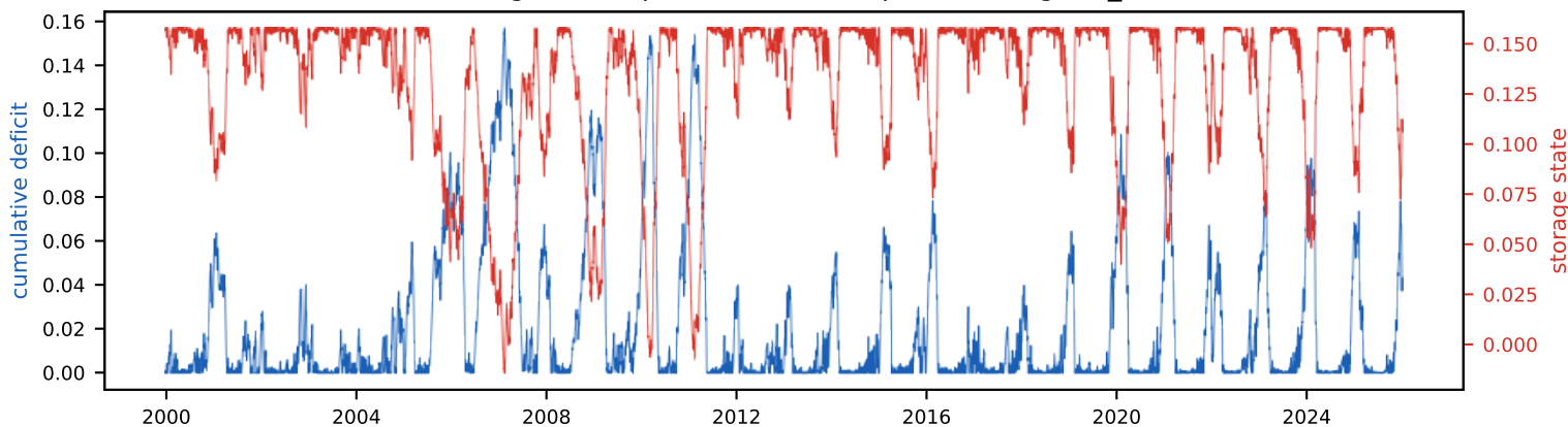
Real energy vs EIA demand (29 TWh/yr, 0.2% land)
