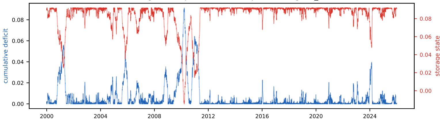
Real energy vs EIA demand (16 TWh/yr, 0.1% land)
