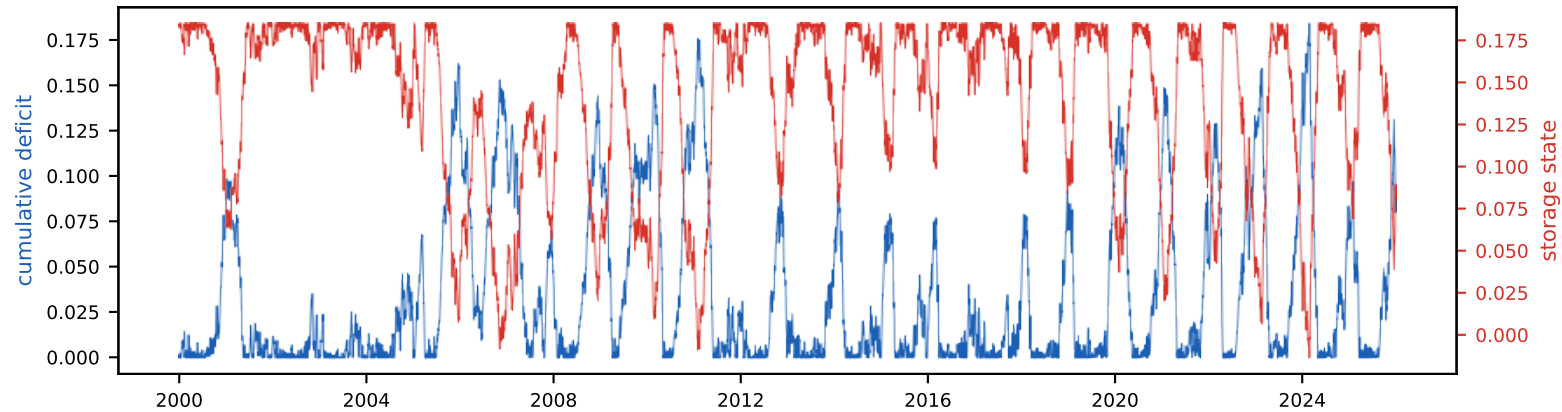
Real energy vs EIA demand (35 TWh/yr, 0.3% land)
