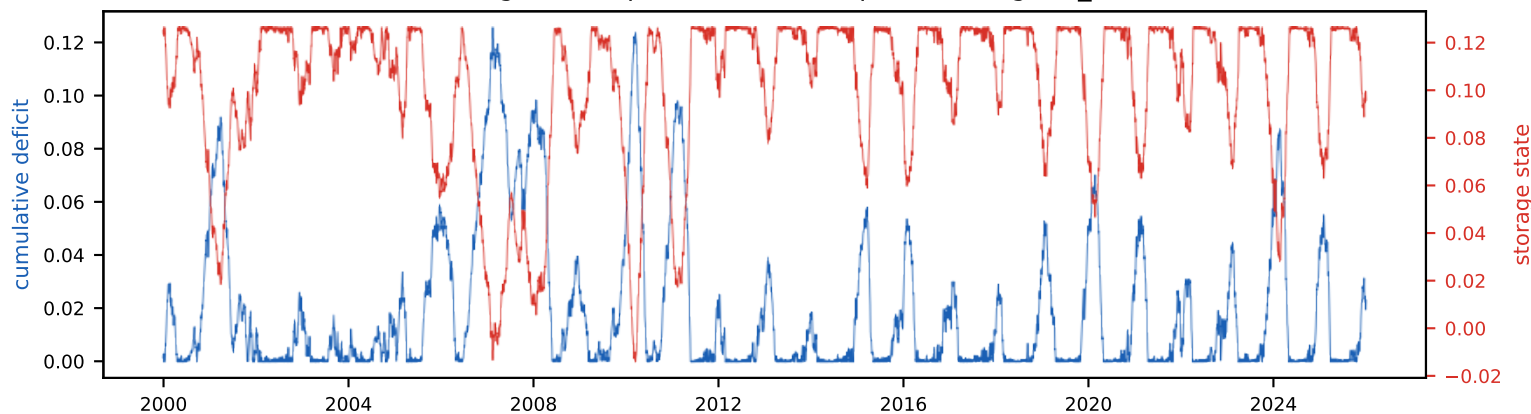
Real energy vs EIA demand (52 TWh/yr, 0.3% land)
